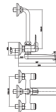
Wall Mixer (Two in One)
