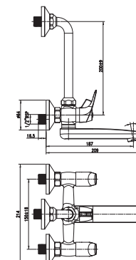
Wall Mixer (Two in One) NEW
